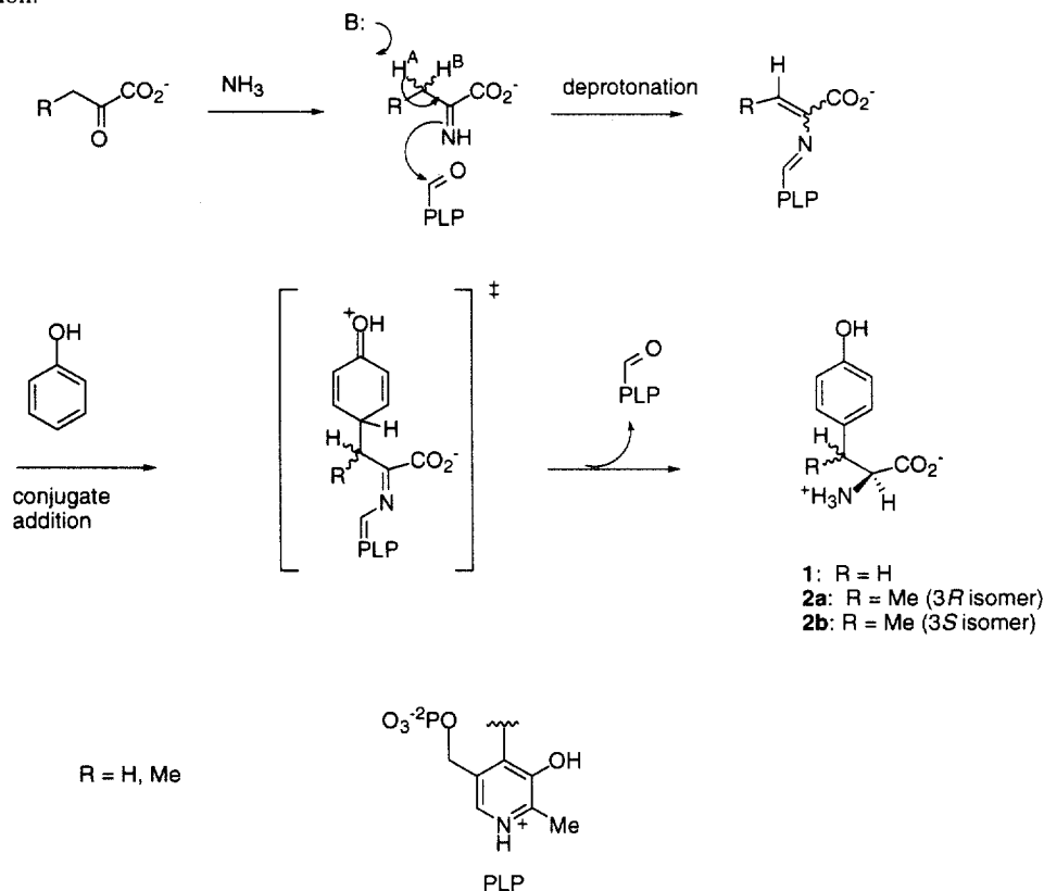
Figure. TPL (Tyrosine Phenol-Lyase) Catalyzed Tyrosine ( 1 ) and \beta -methyltyrosine ( 2 ) Formation
